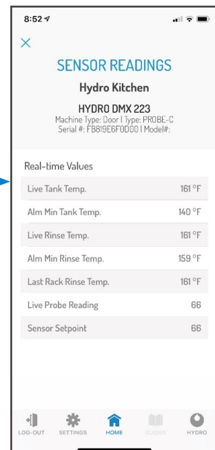
Sensor Readings
